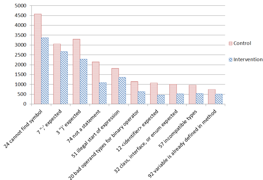
Figure 6. Number of errors per CEM (10 most frequent CEMs enhanced by Decaf).
